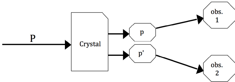
Figure 1: Set-up for observer entanglement experiment. Through the process of Spontaneous Parametric Down-Conversion, a single photon (P) is sent into a crystal and converted into a pair of entangled daughter photons (p and p’), which are then sent to separate observers (obs. 1 and obs. 2).
